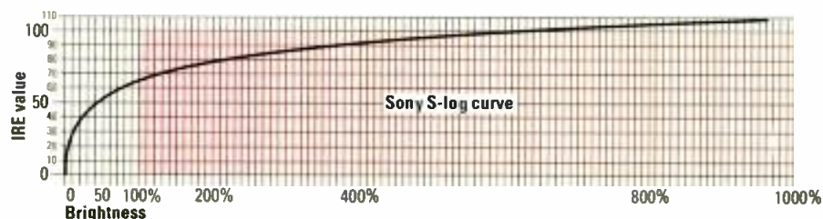
Figure 2. S-log provides 800 percent to 1000 percent greater dynamic range.
